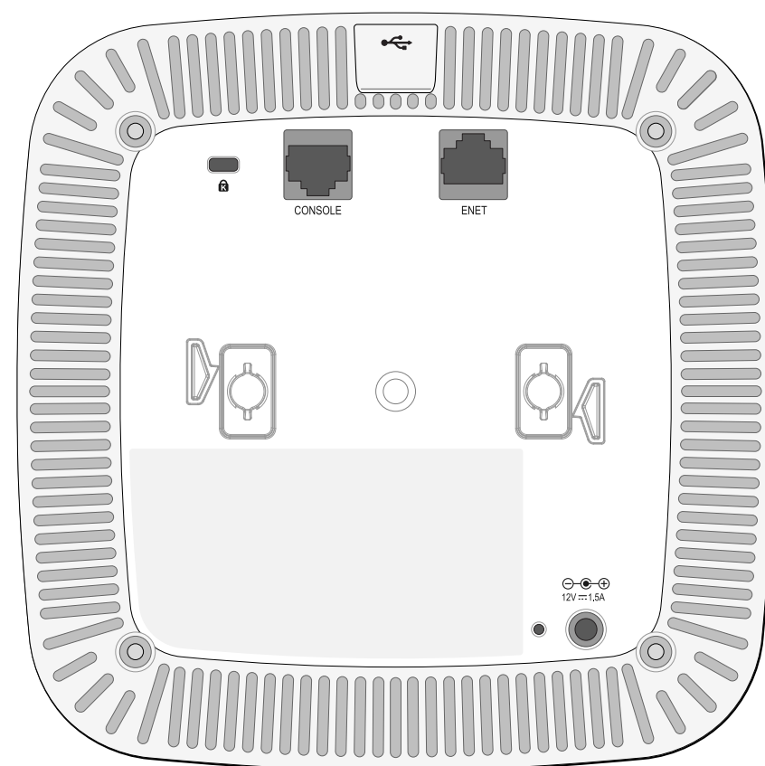
Figure 3 W-IAP110 Series Rear View
