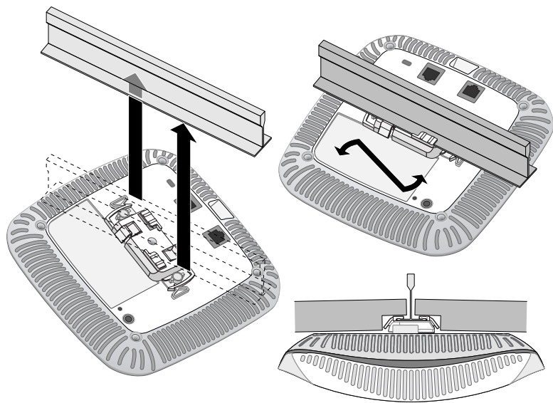
Figure 7 Mounting the IAP
